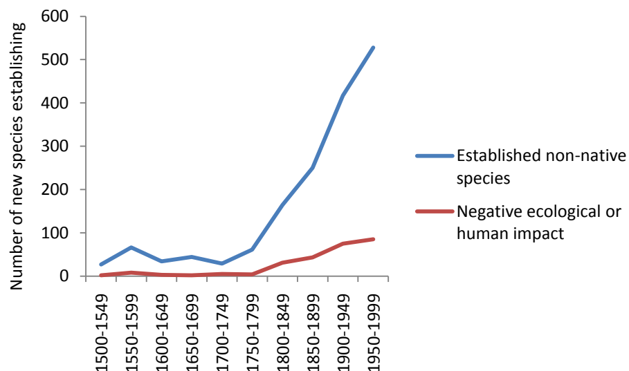
Figure 3. Number of established non-native species and the number that are designated as having a negative ecological or human impact against date of first record. It should be noted that a further 125 species have arrived (only 40 of these are known to have established) between 2000 and 2010 and 14 of these are considered to have a negative impact. There are 170 established non-native species for which there is no date within the species register.
